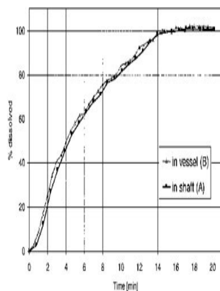
Figure 2: Anticoagulant tablet profile determined in the vessel with the scanning spectrometer and in the hollow shaft with the DAD spectrometer
