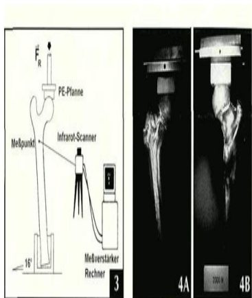
Figure 3: Test apparatus used in the thermoelastic stress analysis. Figure 4: Photoelastic-coating method with strain patterns on intact femurs with two coating methods: medial and lateral (A) and anterior and posterior (B).
